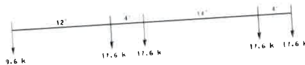
Figure 1: KYTC Standard Analysis Trucks
